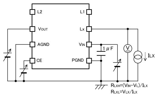
< Circuit No.⑥ >
